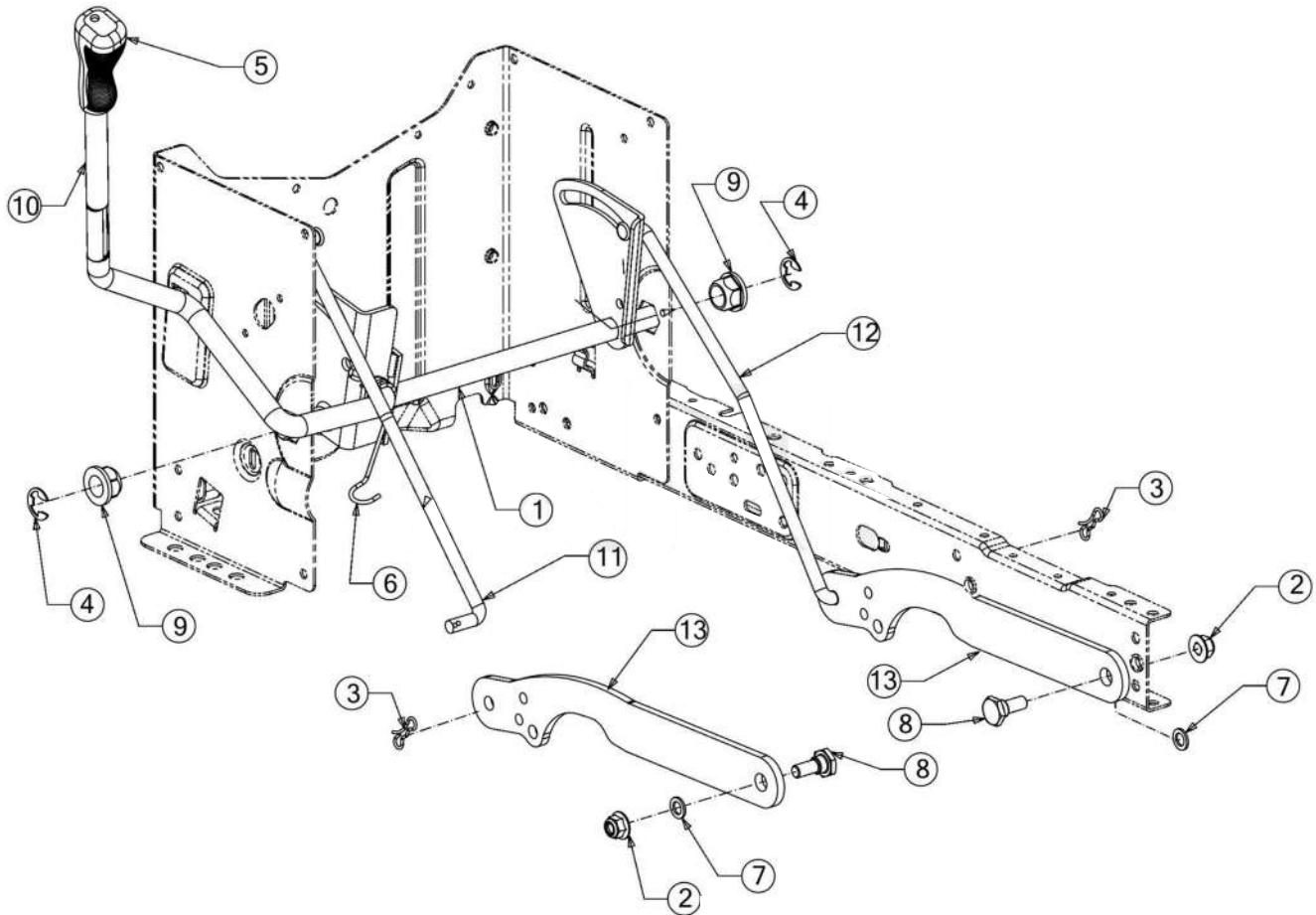
Deck Lift
