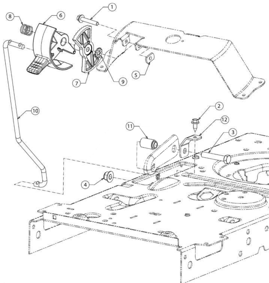
Controls
