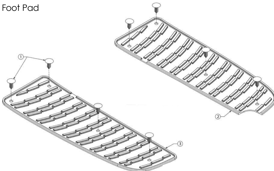
Foot Pad
