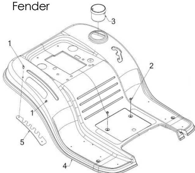
Fender
