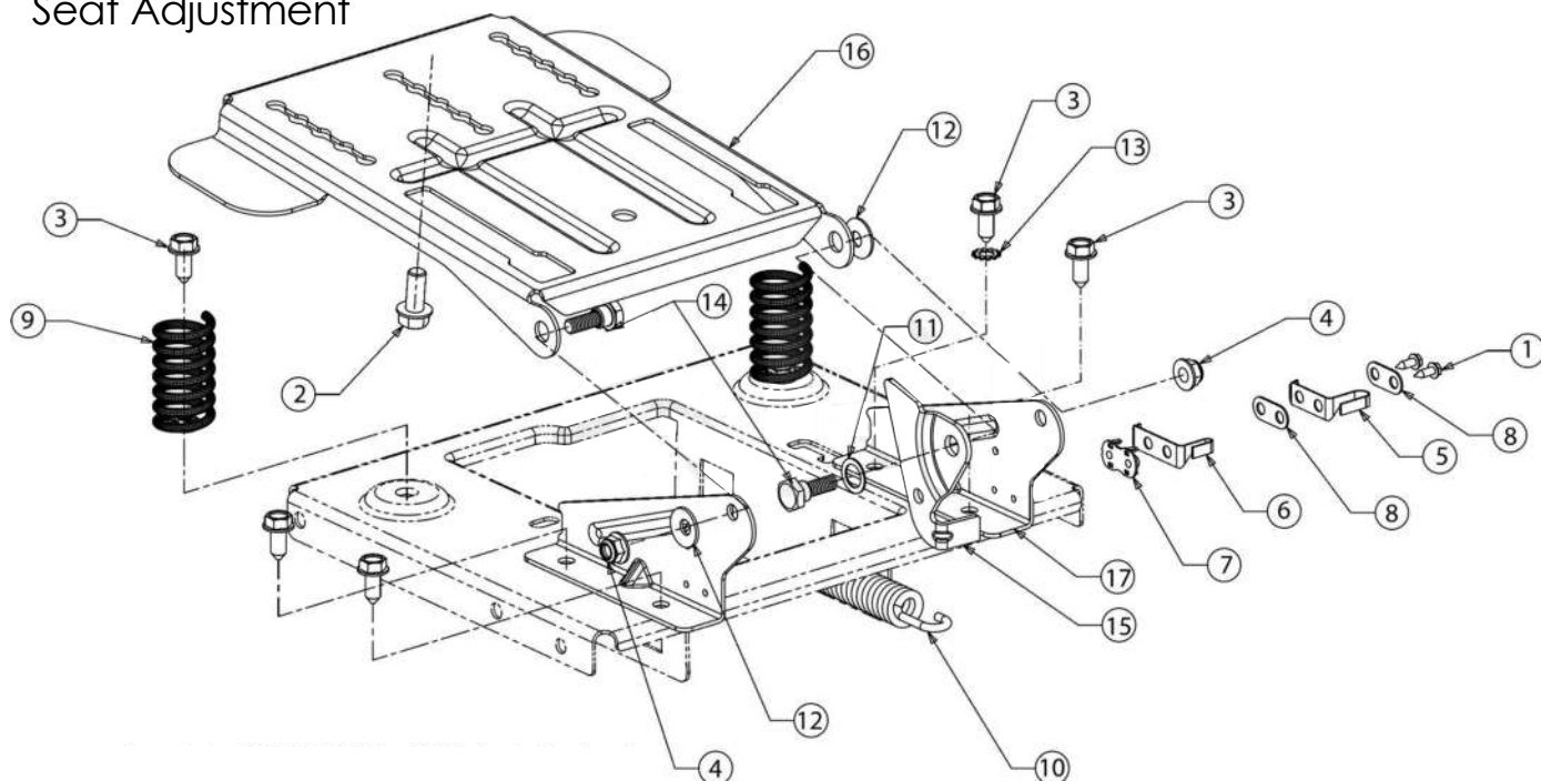
Seat Adjustment
