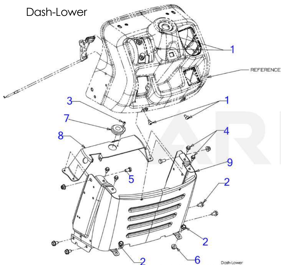
Dash-Lower
