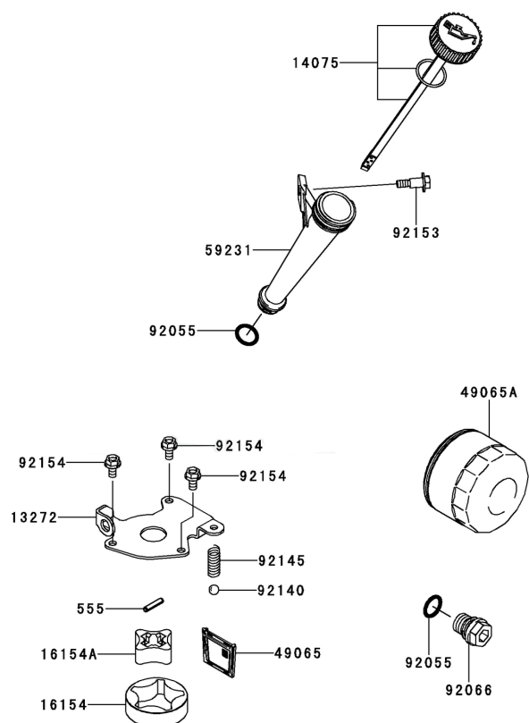
11.LUBRICATION-EQUIPMENT
