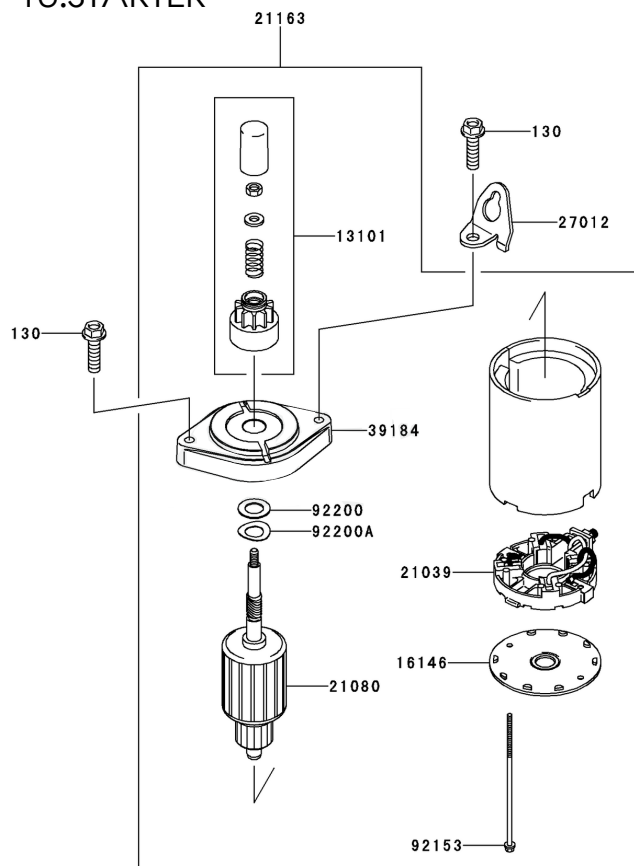
13.STARTER
