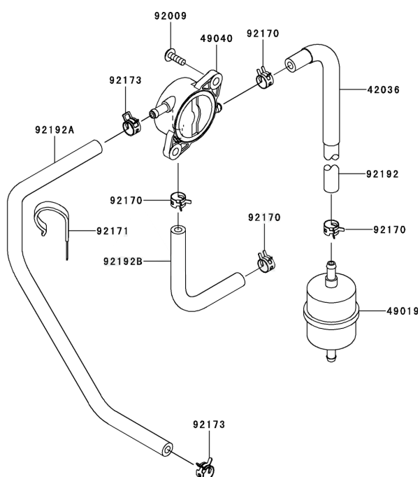
10.FUEL-TANK/FUEL-VALVE
