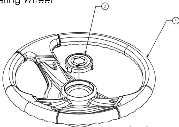
Steering Wheel
